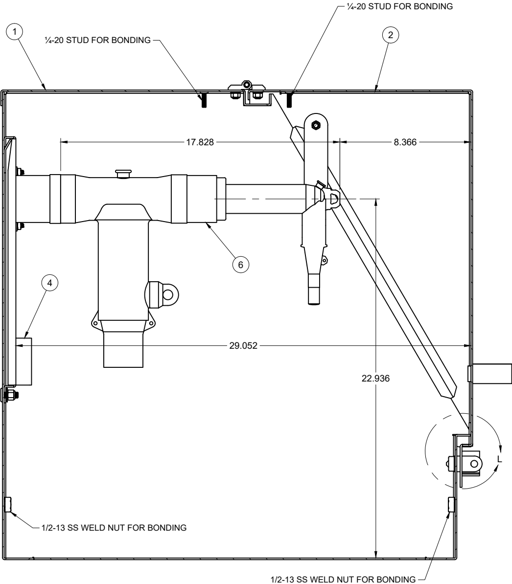
SECTION K-K SCALE 1:6
